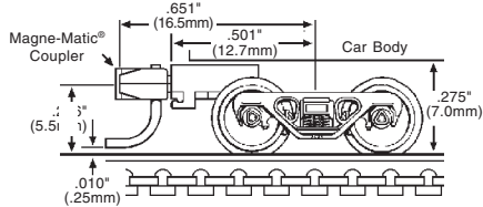
1037-1 BARBER® ROLLER BEARING 003 02 047 with low profile wheels and medium extension mounted Magne-Matic® Coupler
