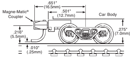
1037 BARBER® ROLLER BEARING 003 02 042 with medium extension mounted Magne-Matic® Coupler
