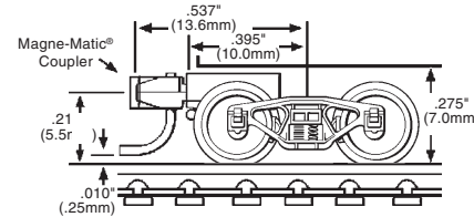
1137 COIL-ELIPTIC 003 02 071 with short extension mounted Magne-Matic® Coupler
