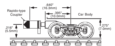
1500 BETTENDORF 003 04 021 with Rapido-type coupler
