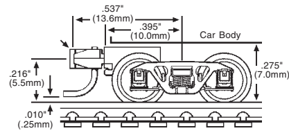
1052 ANDREWS 003 02 011 with short extension mounted Magne-Matic® Coupler
