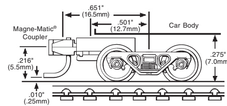
1144 COMMONWEALTH BX 003 02 093 with medium + extension mounted Magne-Matic® Coupler
