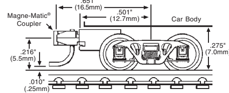
1053 ANDREWS 003 02 012 with medium extension mounted Magne-Matic® Coupler
