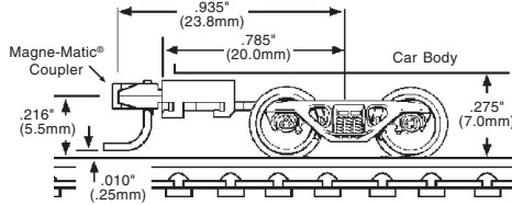
1038 BARBER® ROLLER BEARING 003 02 044 with long extension mounted Magne-Matic® Coupler
