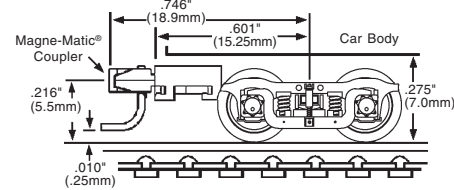
1144 COMMONWEALTH BX 003 02 093 with medium + extension mounted Magne-Matic® Coupler
