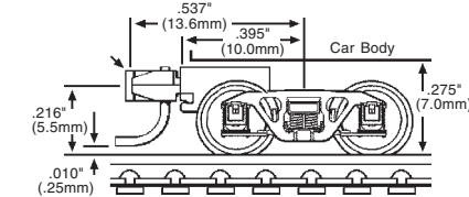
1052-1 ANDREWS 003 02 016 with low profile wheels and short extension mounted Magne-Matic® Coupler
